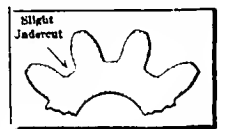
Fig. 5—Segment of 10-tooth, 4-pitch gear
